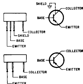
TRANSISTORS PNP
